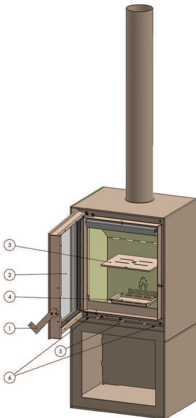
Figure 2: Operation Box with log store
