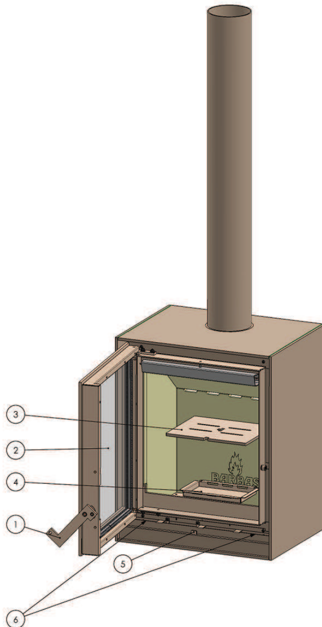
Figure 1: Operation Box
